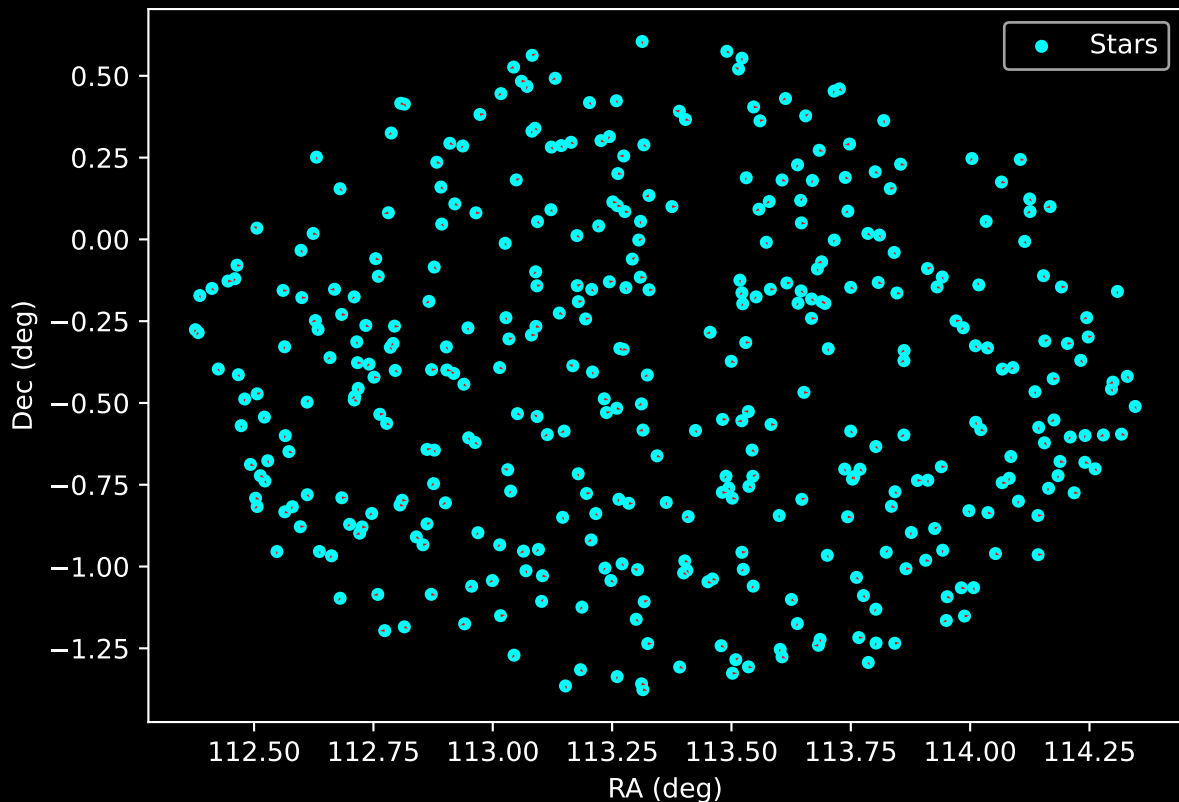
GALAH DR4 Field: [6695] Proper Motion Vectors for Gaia Star Field (n= 377)
