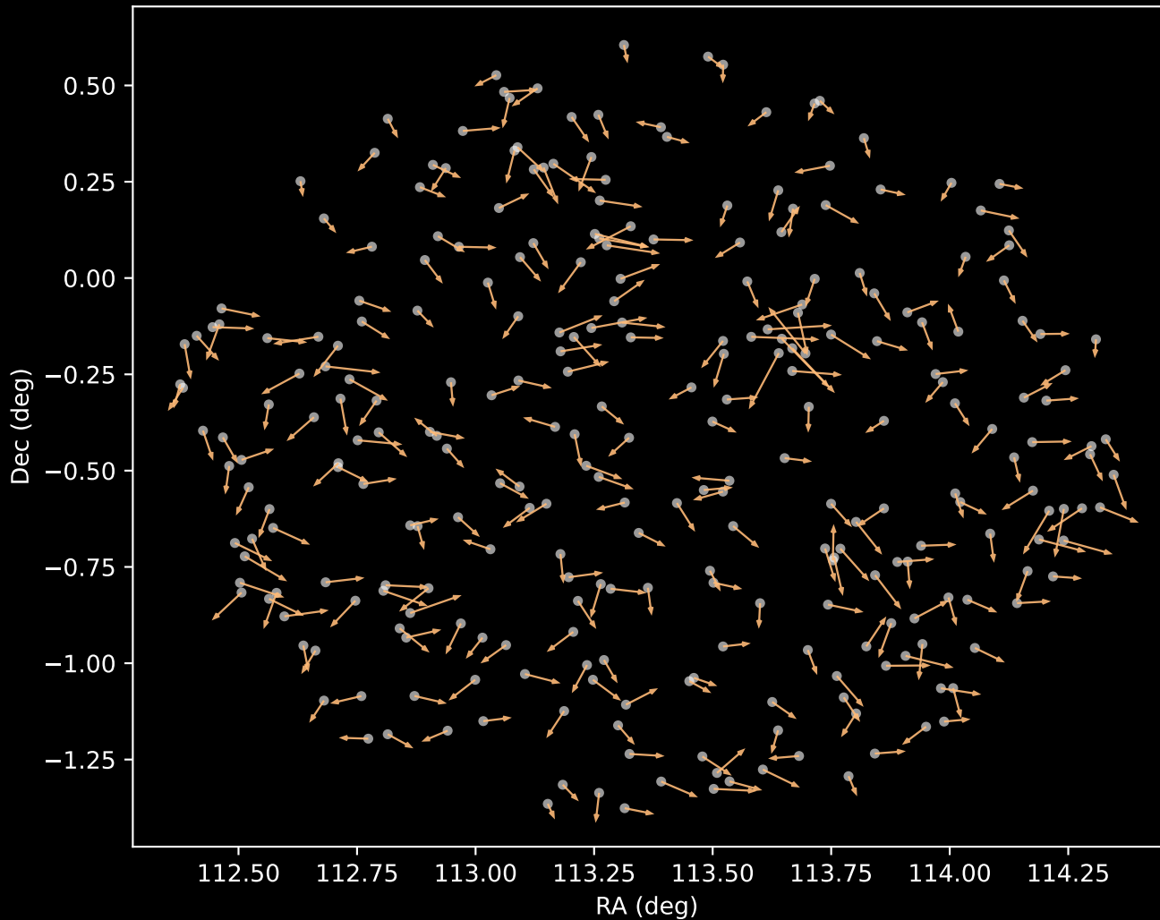
GALAH DR4 Cluster 3 Proper Motion Vectors (n=278)
