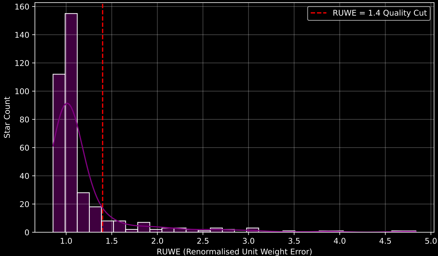
GALAH DR4 Field [6695] RUWE Distribution (n= 362)
