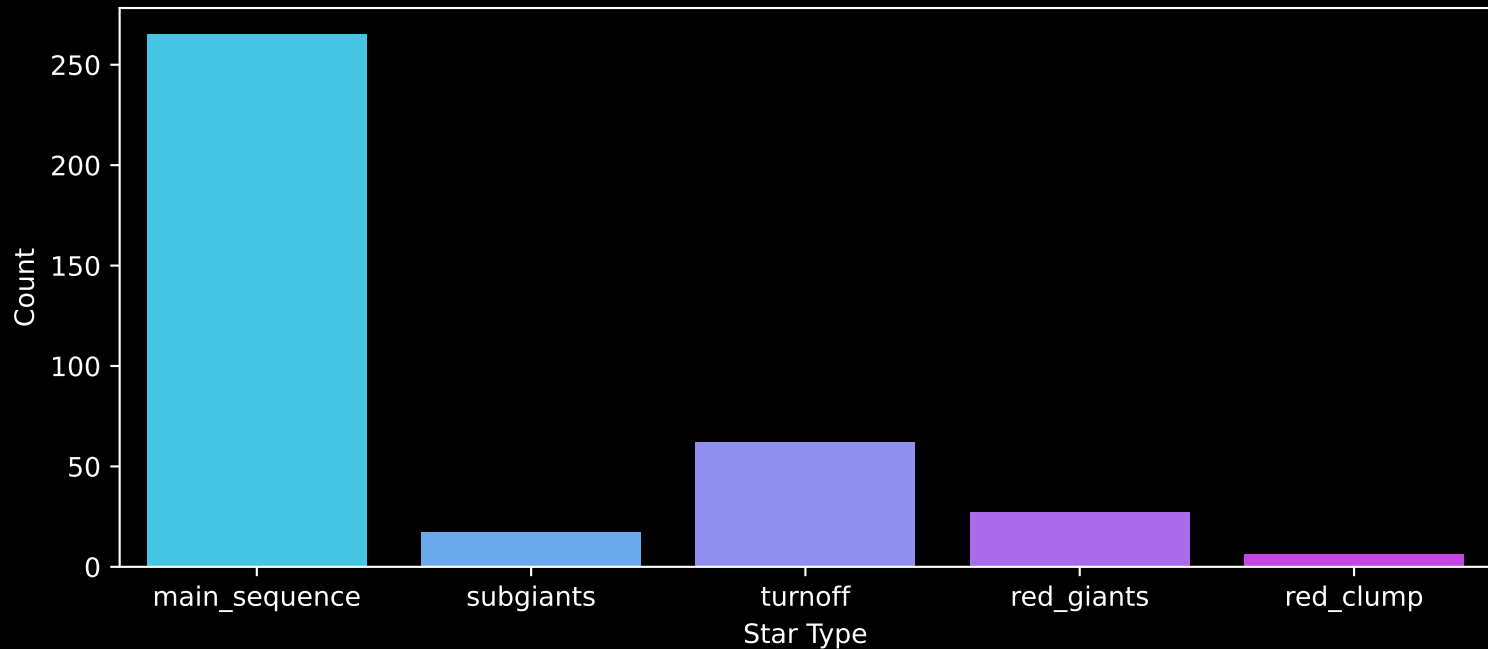
GALAH DR4 Field: [6695] Count plot of Star Type
